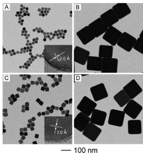
Figure 1. TEM images of two different types of single-crystal Ag seeds and Ag nanocubes obtained from these seeds: (A,B) spherical seeds and the resultant nanocubes and (C,D) cubic seeds and the resultant nanocubes. In a typical synthesis, 200 \mu\text{L} of \text{AgNO}_3 (282 mM) was added to 50 \mu\text{L} of spherical ( 1.1 \times 10^{12} particles/mL) or cubic ( 1.1 \times 10^{12} particles/mL) seeds, and the reaction was terminated in 3 h.
