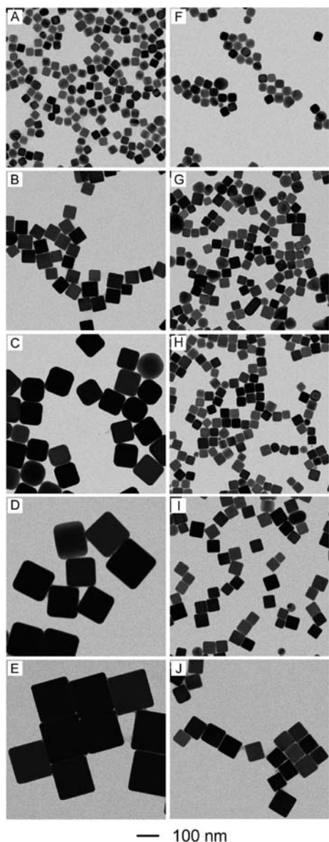
Figure 4. Size control over Ag nanocubes by adding different amounts of \text{AgNO}_3 (left column) and single-crystal seeds (right column): (A–E) 10, 50, 75, 100, and 200 \mu\text{L} of \text{AgNO}_3 was added to 50 \mu\text{L} of spherical seeds ( 1.1 \times 10^{12} particles/mL); (F–J) 300, 200, 100, 50, and 20 \mu\text{L} of the spherical seeds ( 1.1 \times 10^{12} particles/mL) was used with 50 \mu\text{L} of \text{AgNO}_3 solution (282 mM).
