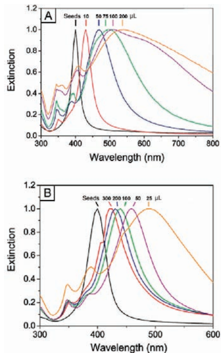
Figure 5. UV–vis spectra taken from products of the syntheses shown in Figure 4: (A) adding different amounts (as indicated on the curves) of \text{AgNO}_3 to the same amount of spherical seeds and (B) adding different amounts (as indicated on the curves) of spherical seeds to the same amount of \text{AgNO}_3 solution.
