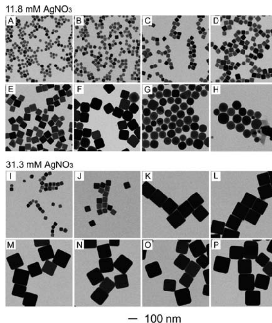
Figure 2. TEM images of samples obtained at different stages of two syntheses, where the same amount of seeds (spherical, 50 \mu\text{L} , and 1.1 \times 10^{12} particles/mL) was used but \text{AgNO}_3 solutions of two different concentrations, 11.8 and 31.3 mM, were used: (A,I) 10 min, (B,J) 20 min, (C,K) 40 min, (D,L) 1 h, (E,M) 2 h, (F,N) 3 h, (G,O) 4 h, and (H,P) 5 h.
